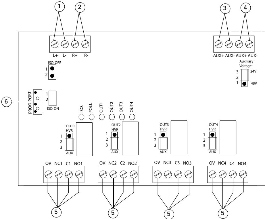
Fig. 3: Terminal Arrangement
