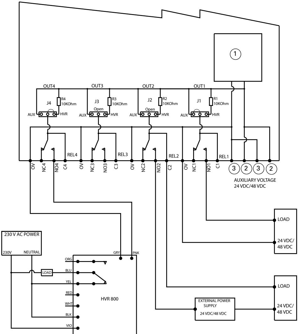
Fig. 4: Terminals
