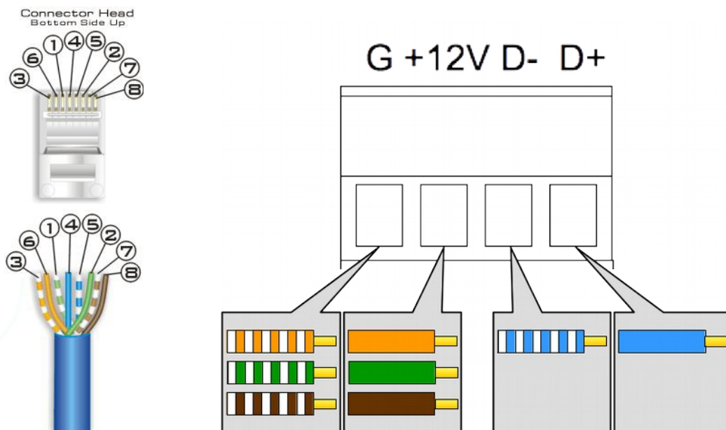
Illustration 6: VCC-64 PSK to VCC-64 connection detail
