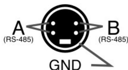
Illustration 3: Serial Input Port (mini-DIN 4 female)
