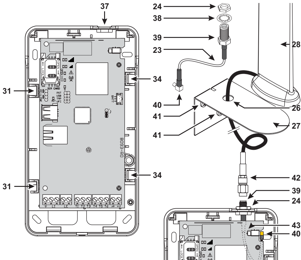
Figure 5 – Installation de l'antenne ANTLTE-02.
