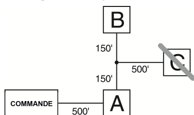
Figure 1-1 Câblage Corbus
