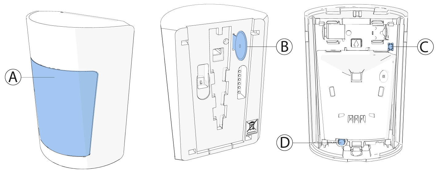
Figure 1: MP-802 PG+
