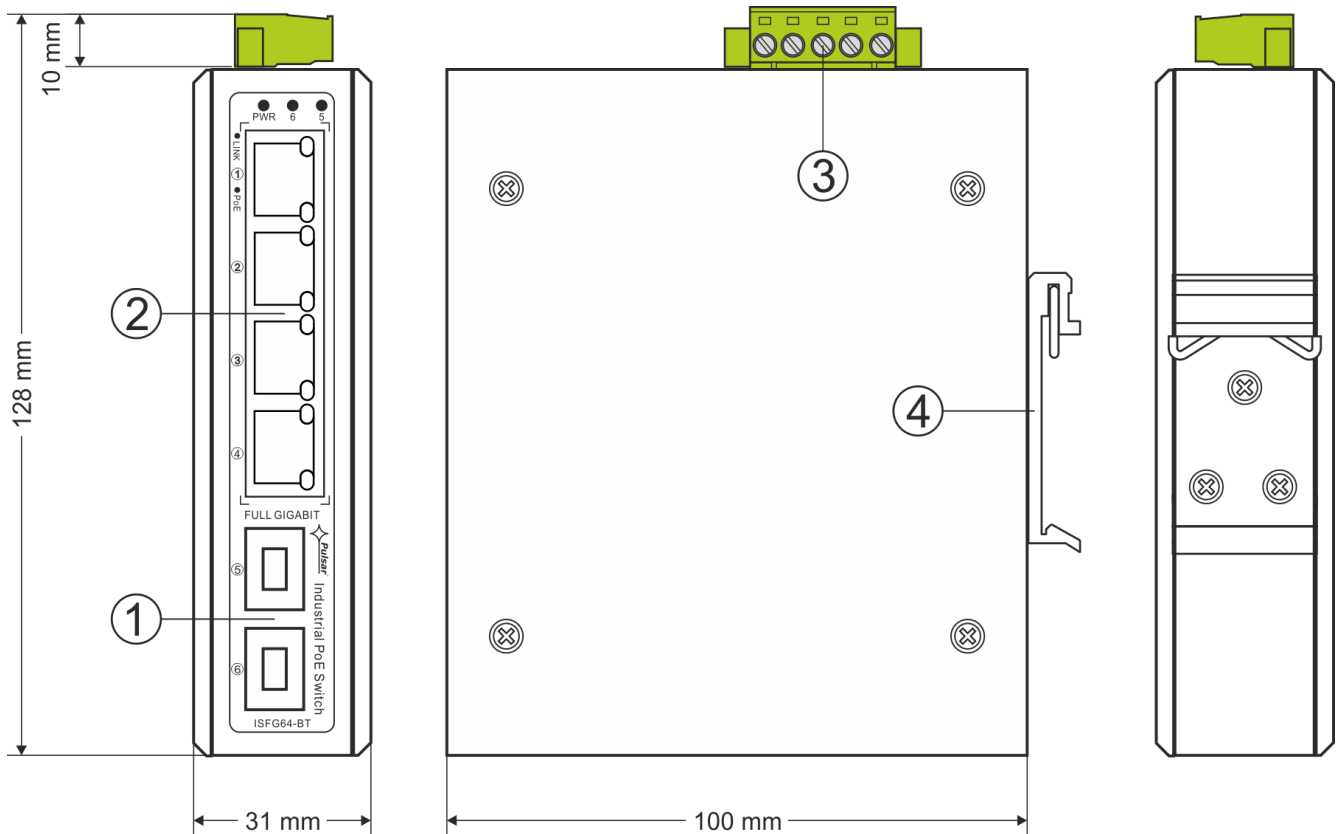
Fig. 2. View of the switch.
